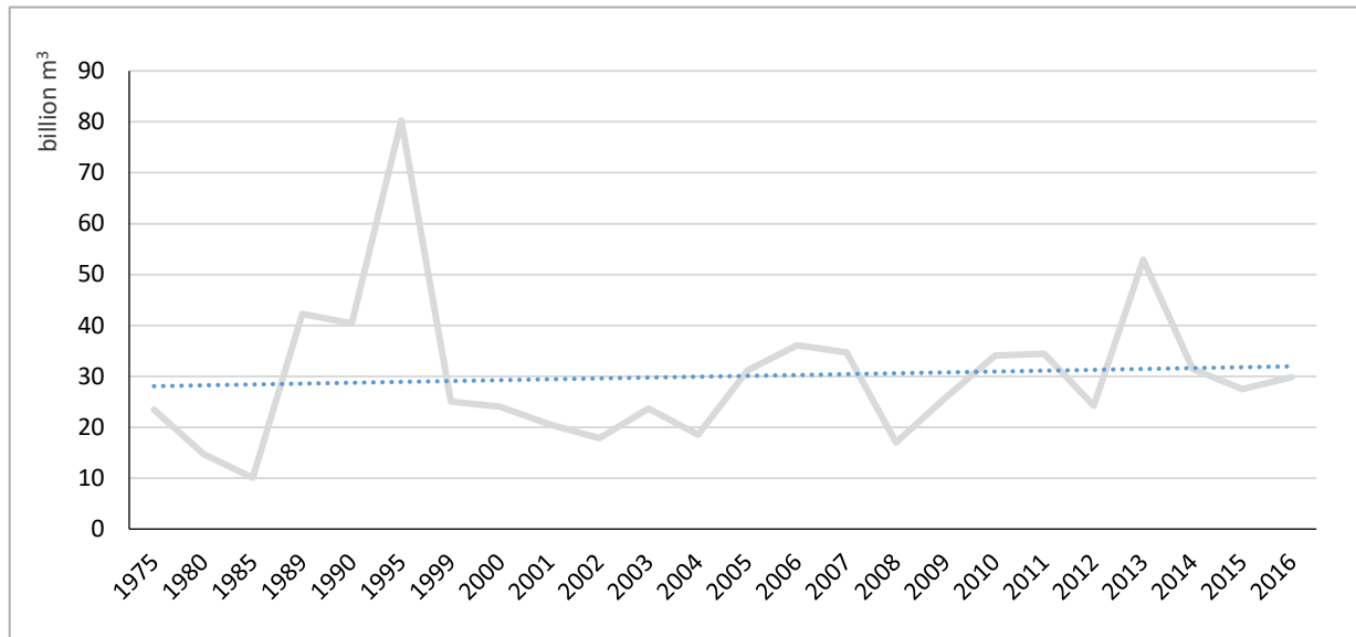
Figure 16: Precipitation in Sultanate of Oman from 1975 to 2016
